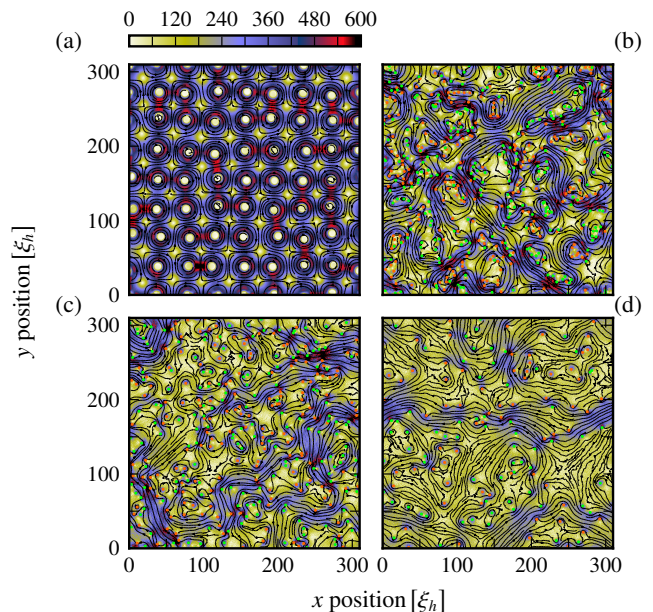
FIG. 2. The hydrodynamic velocity field \mathbf{v} corresponding to the snapshots of the time evolving density shown in Fig. 1. Black flow lines indicate the orientation of the velocity field while the color projection depicts the modulus |\mathbf{v}| . The positions of elementary vortices (anti-vortices) in panels (b)–(d) are marked by orange (green) dots. The strong clustering after the initial break-up as well as the large-scale vortex clustering leading to strong coherent flows during the universal, late-time stage are clearly seen. For comparison we provide corresponding flow diagrams for the evolution near the dissipative (Gaussian) fixed point in Appendix B.
