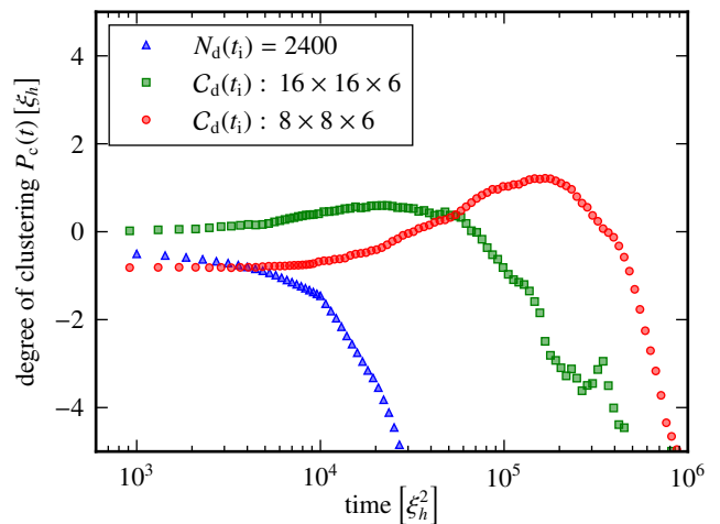
FIG. 9. Degree P_c(t) of clustering of elementary like-sign vortices as a function of time, defined in Eq. (32), for the same three initial conditions as used in Fig. 7. Deviations of P_c from zero indicate clustering ( P_c > 0 ) or anti-clustering ( P_c < 0 ). A strong anti-clustering of like-sign defects, such as for the data marked by (blue) triangles, is accompanied by vortex–anti-vortex pairing.
