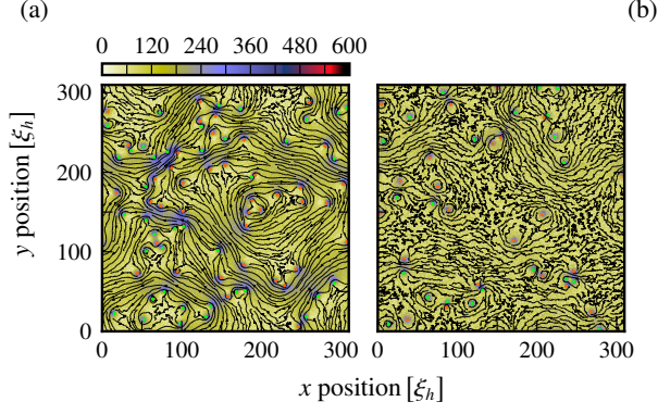
FIG. C.1. The hydrodynamic velocity field \mathbf{v} corresponding to the snapshots of the time evolving density shown in Fig. 1 (panel a). Black flow lines indicate the orientation of the velocity field while the colour projection depicts the modulus |\mathbf{v}| . The positions of vortices (anti-vortices) are marked by orange (green) dots. The strong clustering after the initial break-up as well as the large-scale vortex clustering leading to strong coherent flows during the universal, late-time stage are clearly seen. Panel b shows a characteristic hydrodynamic velocity field near the Gaussian non-thermal fixed point. Here, the system largely consists of relatively closely bound pairs of vortices and anti-vortices. Both flow fields are depicted at a time t = 4 \cdot 10^4 \xi_h^2 .
