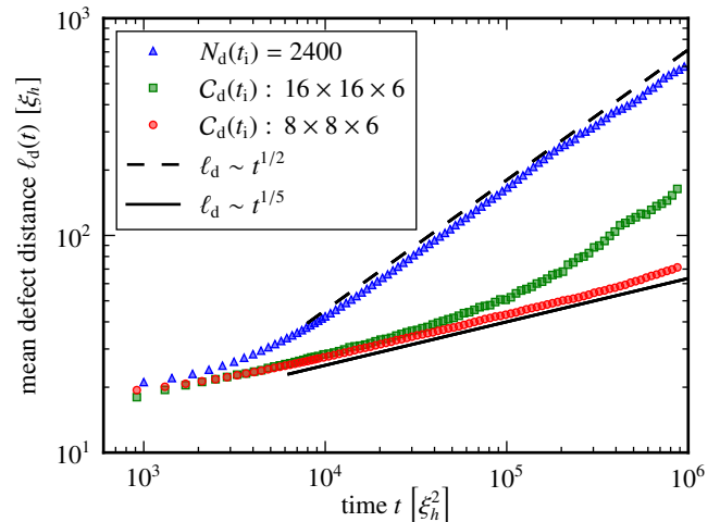
FIG. 7. Mean defect distance \ell_d as function of time, after phase-imprinting different initial vortex configurations at t_i = 0 . The (blue) triangles show the evolution from a random distribution of N_d(t_i) = 2400 elementary vortices and anti-vortices (total angular momentum zero), corresponding to the evolution shown in Fig. 6. The (green) squares and (red) circles show the evolution from an irregular square lattice of 16 \times 16 and 8 \times 8 non-elementary vortices with winding numbers w = \pm 6 , see Fig. 1a for an example. The evolution marked by the (red) circles corresponds to Fig. 4. As indicated by the dashed and solid black lines, the growth of the distance is well approximated by power laws \ell_d(t) \sim t^{\beta_d} with \beta_d = 1/2 (Gaussian fixed point) and \beta_d = 1/5 (anomalous fixed point), respectively. As indicated by the evolution marked by the (green) squares, depending on the initial conditions, the system can first approach the anomalous fixed point before it turns to steeper scaling near the Gaussian one.
