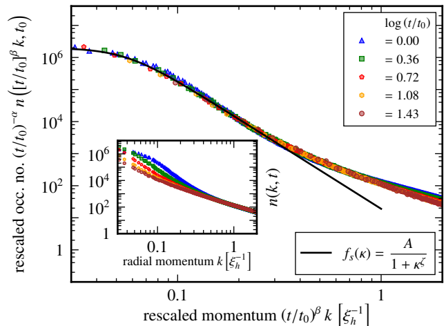
FIG. 6. The graphs illustrate the scaling analysis of the evolution close to the Gaussian non-thermal fixed point as shown in Fig. 5, in full analogy with Fig. 4. The reference time is, again, t_0 = 10^4 \xi_h^2 . The scaling exponents are determined to be \alpha = 1.10 \pm 0.08 and \beta = 0.56 \pm 0.08 . The scaling function (black line) exhibits a Porod-law exponent \zeta = 4.0 \pm 0.1 .
