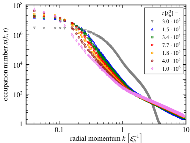
FIG. 3. Single-particle momentum spectrum at seven, logarithmically equidistant times starting from the initial configuration bearing an (8 \times 8) -lattice of non-elementary vortices with winding number w = \pm 6 , as exemplary shown in Figs. 1 and 2. After the initial build-up of a characteristic distribution, a self-similar shift towards smaller momenta is seen during the universal stage of the time evolution. This inverse transport process conserves particle number and, as compared to a turbulent cascade, is non-local in momentum space. The earliest time shown ( t = 3 \cdot 10^2 \xi_h^2 , grey points) is still within the non-universal stage of evolution right after the decay of the lattice ( cf. Fig. 1b). The dynamics during the later stage of the evolution represents a rescaling in space and time and is analyzed in more detail in Fig. 4.
