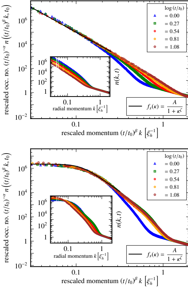
FIG. C.2. Scaling analysis of the time evolving single-particle spectra for the vortex lattice initial condition with 8 vortices of winding number w = \pm 6 , when coupled to a thermal bath with \delta = 0.00215 at temperature T = 100\xi_h^{-2} . Upper panel : Scaling collapse at late times, in the interval 1 \cdot 10^4 \xi_h^2 < t < 1 \cdot 10^5 \xi_h^2 . The inset shows the non-rescaled spectra at five different, logarithmically equidistant times as given in the legend. The times are defined relative to the reference time t_0 = 1 \cdot 10^4 \xi_h^2 . The main graph depicts the scaling collapse of the spectrum according to n(k, t) = (t/t_0)^{-\alpha} n([t/t_0]^\beta k, t_0) . The corresponding scaling exponents, determined from a fit of 100 logarithmically equidistant times, are \alpha = 1.2 \pm 0.05 and \beta = 0.53 \pm 0.05 . The universal scaling function in this time interval does not display the cut-off of the scaling form k_\lambda any more, as it is beyond the infrared cut-off of the computational grid. However, we determine a scaling exponent \zeta = 4.0 \pm 0.1 from fitting a power law to the infrared part of the rescaled spectra (cf. Appendix D). Lower panel : Same analysis as above for the time interval 2 \cdot 10^2 \xi_h^2 < t < 2 \cdot 10^3 \xi_h^2 . The corresponding scaling exponents, determined from a fit of 100 logarithmically equidistant times, are \alpha = 0.41 \pm 0.05 and \beta = 0.22 \pm 0.05 . The universal scaling form in this time interval is consistent with that near the anomalous fixed point in the isolated system, with a scaling exponent \zeta = 5.7 \pm 0.1 .
