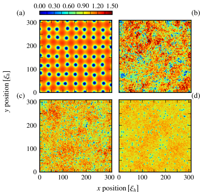
FIG. 1. Time evolution of a 2D superfluid in a square volume with periodic boundary conditions, starting from a lattice of non-elementary vortices with alternating winding numbers w = \pm 6 , arranged in a checker-board manner (panel (a)). Color encodes the superfluid density normalized to the mean density, |\phi|^2/\rho . The vortices quickly break up into clusters of elementary defects with w = \pm 1 . This decay is enhanced by the slight initial displacements of the defects with respect to the square lattice. Panels (b)–(d) show snapshots of the evolving density at times t = \{300, 10^3, 10^4\} \xi_h^2 . In the early non-universal stage of the time evolution (panel (b)), the vortex configuration is strongly clustered. During the later stages shown exemplarily in (c) and (d), the vortices and anti-vortices mutually annihilate in a way that the vortex number falls off in a universal manner as N(t) \sim t^{-2/5} (see main text).
