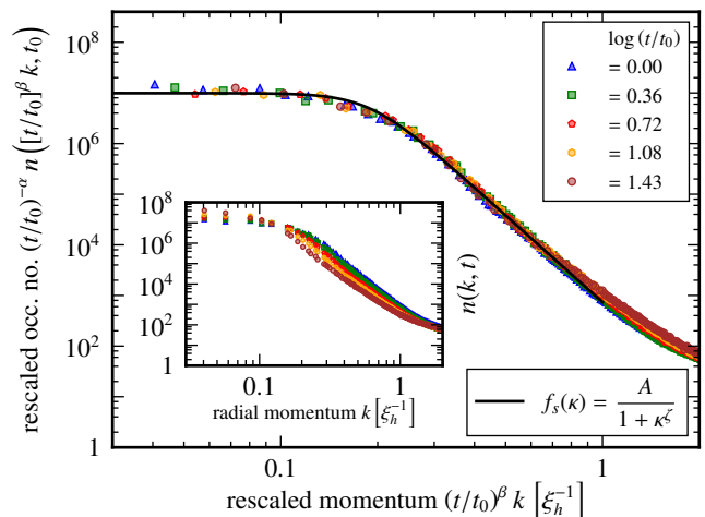
FIG. 4. Scaling analysis of the time evolving single-particle spectra shown in Fig. 3, exhibiting the scaling at the anomalous non-thermal fixed point. The inset shows the non-rescaled spectra at five different, logarithmically equidistant times as given in the legend. The times are defined relative to the reference time t_0 = 10^4 \xi_h^2 , such that the latest time is t = t_0 \cdot 10^{1.43} = 2.7 \cdot 10^5 \xi_h^2 . The main graph depicts the scaling collapse of the spectrum according to n(k, t) = (t/t_0)^{-\alpha} n([t/t_0]^\beta k, t_0) . The respective scaling exponents are determined by a fit which yields \alpha = 0.402 \pm 0.05 and \beta = 0.193 \pm 0.05 . The functional form (19) is fit to the scaling function (black line) and shows a Porod-tail scaling exponent \zeta = 5.7 \pm 0.3 . For a better visibility we show only five exemplary curves, while the scaling-collapse fits involve the whole data set, consisting of spectra at 300 logarithmically equidistant times within the universal stage of the evolution.
