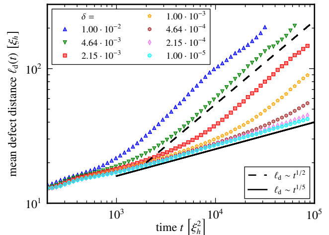
FIG. 8. Mean defect distance \ell_d as function of time, after preparing an irregular 8 \times 8 square lattice of non-elementary (anti-)vortices with winding number w = \pm 6 . Symbols (colors) mark the evolution for different parameters \delta and \gamma , describing the coupling to the bath, cf. Eq. (C.5), in a way that the temperature is held fixed at T = 2k_B\delta/\gamma = 100\xi_h^{-2} . Comparing with Fig. 7 we find the same universal growth laws \ell_d(t) \sim t^{\beta_d} near the anomalous fixed point ( \beta_d = 1/5 ) and near the Gaussian fixed point ( \beta_d = 1/2 ) as for the isolated system. Moreover, the crossover time scale from anomalous to Gaussian scaling is controlled by the strength of the coupling \delta to the thermal bath. This suggests that also through the different initial conditions chosen in Fig. 7, a thermal bath is created which eventually forces the system to deviate from the anomalous fixed point. At late times, the data is limited by averaging statistics while at least one vortex–anti-vortex pair is left.
