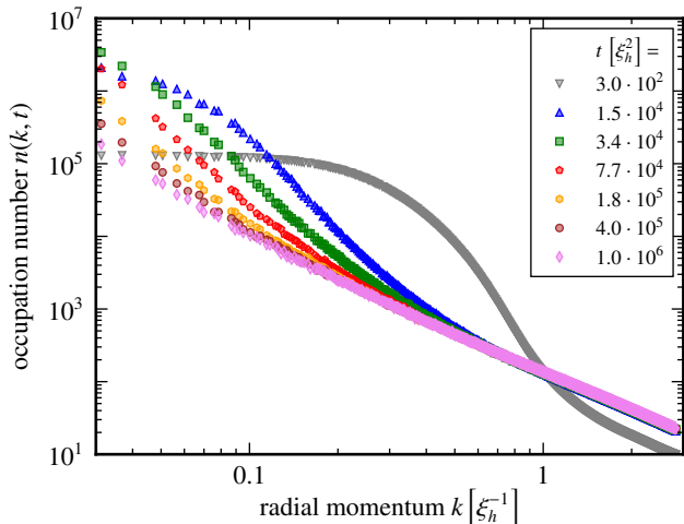
FIG. 5. Single-particle momentum spectrum at seven, logarithmically equidistant times starting from the initial configuration bearing a random distribution of 2400 elementary vortices with winding number w = \pm 1 , summing to a total angular momentum zero. After the initial build-up of a characteristic distribution, a self-similar shift towards smaller momentum scales is seen during the universal stage of the time evolution. The earliest time shown ( t = 3 \cdot 10^2 \xi_h^2 , grey points) is still within the non-universal stage. The scaling during the later universal stage is analyzed in Fig. 6.
